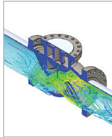
Flow simulation
